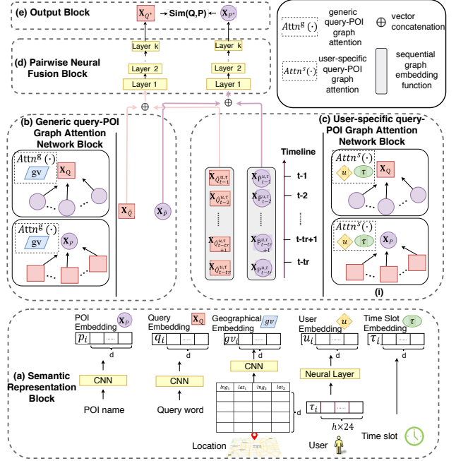
Figure 3: Framework overview.
